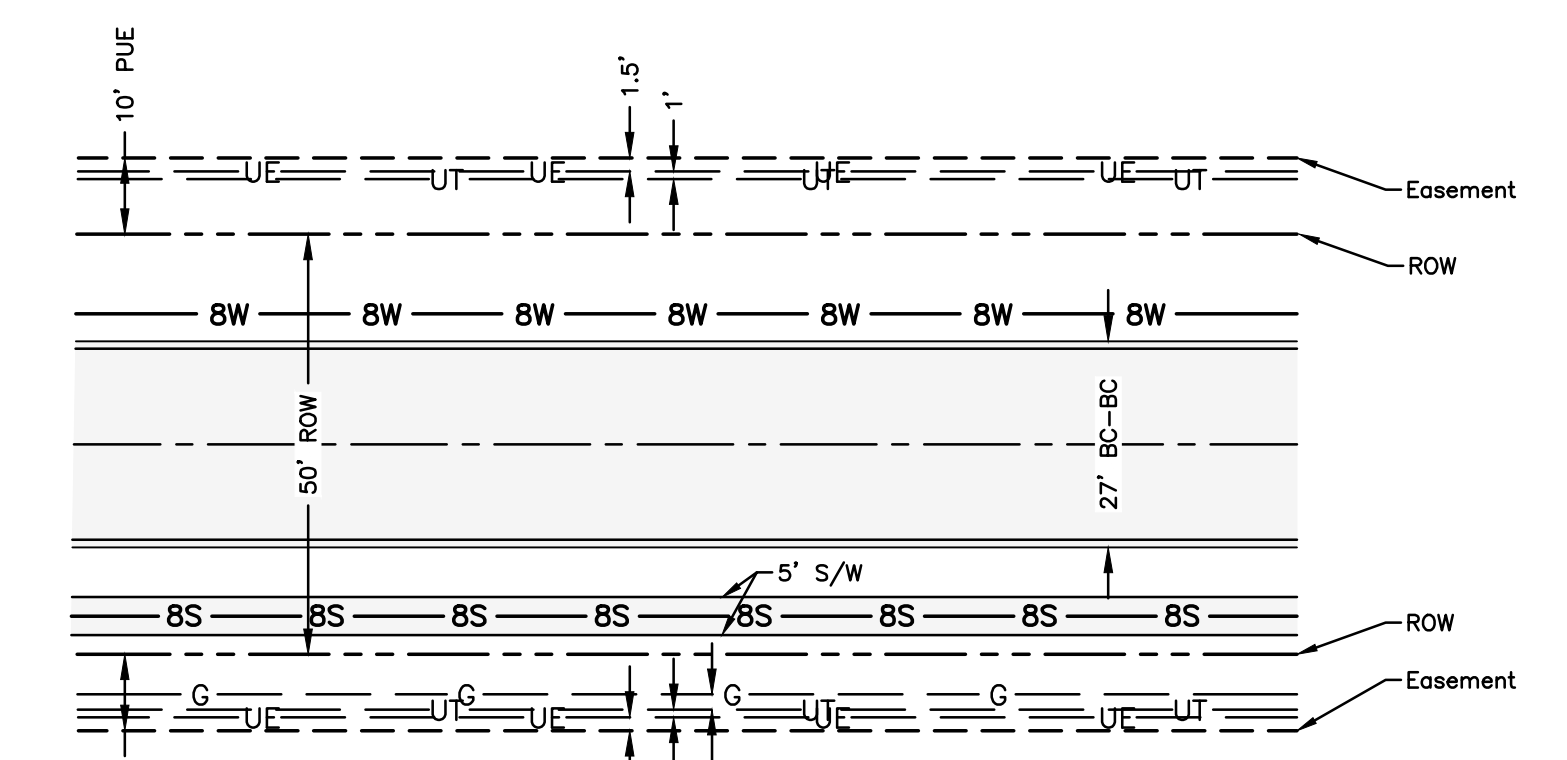
NOTE: This serves as a general guide only. Utility Company is to provide location of proposed electric, gas, and telecommunication lines. Typical Utility Layout
